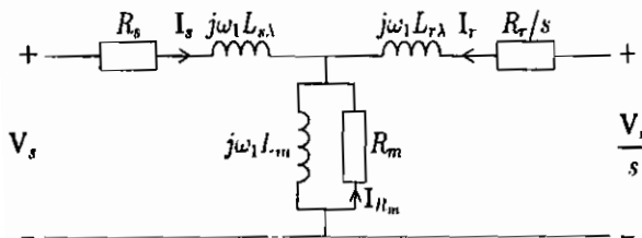
Fig. 2: Equivalent Circuit of the DFIG
