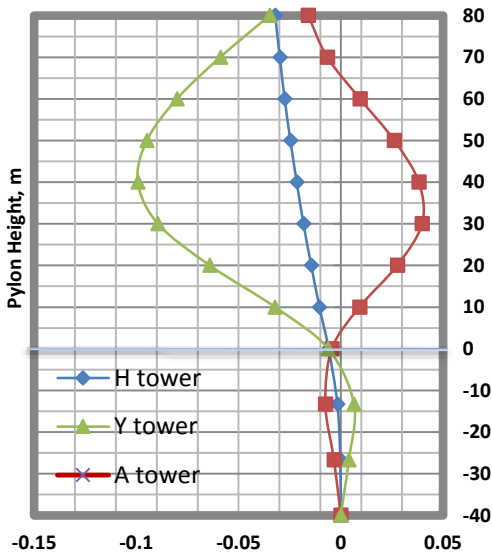
Fig. (29): Sway Y, Case A, Radiating.
