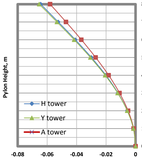
Fig. (34): Sway X, Case D, Radiating.
