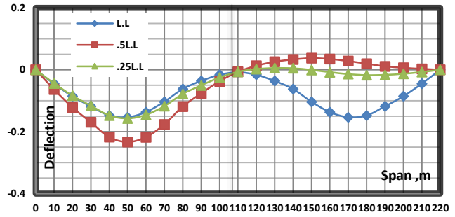
Fig. (44): Deflection, Case A, Harp.
