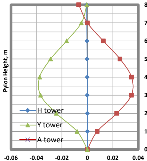
Fig. (35): Sway Y, Case D, Radiating.
